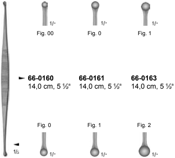
MARTINI 66-0160 - 66-0163
